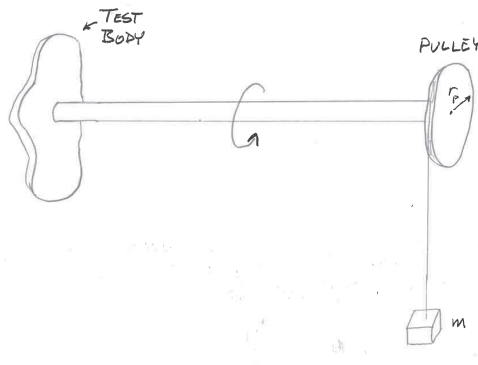
Figure 39.1: A simple device for measuring the moment of inertia.
