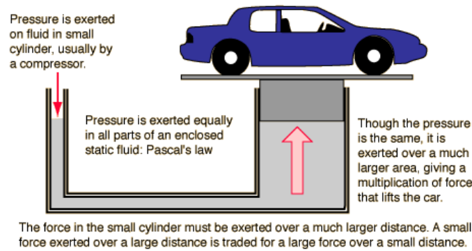
Figure 53.2: An automobile on a hydraulic press. (Credit: HyperPhysics project, Georgia State University, Ref. [9]).
