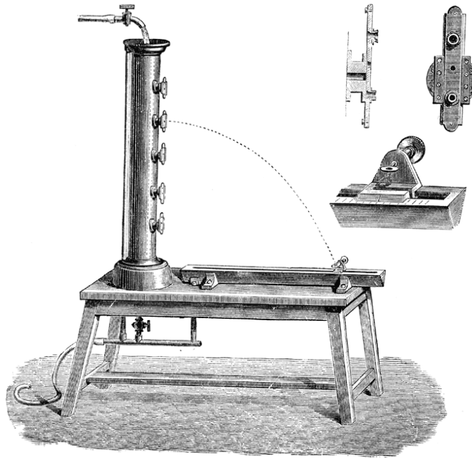
Figure 52.2: Apparatus for demonstrating Torricelli's theorem. (Ref. [16])
