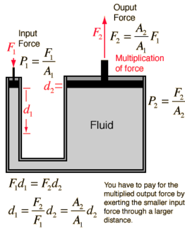
Figure 53.1: The hydraulic press. (Credit: HyperPhysics project, Georgia State University, Ref. [9]).
