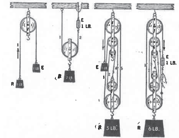
Figure 25.3: Systems of pulleys. These systems have a mechanical advantage of (left to right): 1, 2, 5, and 6, so that each example requires only 1 lb of effort to lift 1, 2, 5, and 6 pounds, respectively. Note that the leftmost arrangement only changes the direction of the applied effort force, by allowing us to pull downward to lift the weight upward; it does not provide any mechanical advantage. (Ref. [19])
