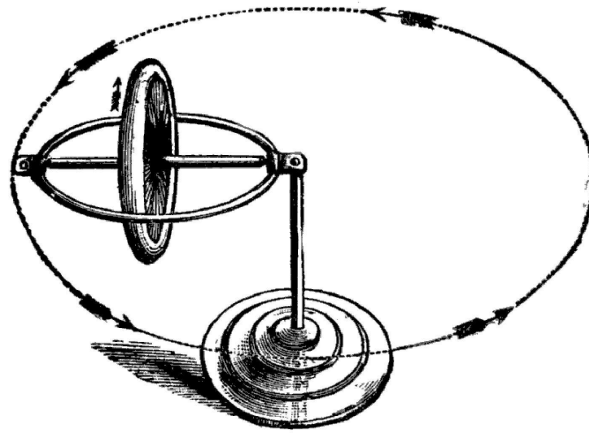
Figure 49.1: Motion of a gyroscope. By the right-hand rule, the angular momentum of the wheel is to the left. The torque vector due to the gyroscope tipping over is horizontal, toward the observer. This torque vector “pushes” the angular momentum vector around counterclockwise, as shown; the resulting motion is called precession . (From Ref. [15])
