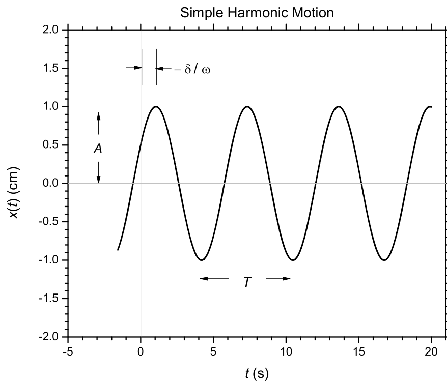
Figure 42.1: Simple harmonic motion. Shown are the amplitude A , period T , and phase constant \delta . The horizontal line x(t) = 0 is the equilibrium position.
