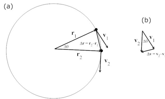
Figure 23.1: (a) A body moving in a circular path of radius r with constant speed v . At time t_1 , the body is at position \mathbf{r}_1 and has velocity \mathbf{v}_1 ; at a slightly later time t_2 , it is at position \mathbf{r}_2 and has velocity \mathbf{v}_2 . (b) The difference in velocity vectors \mathbf{v}_2 - \mathbf{v}_1 is the direction of the acceleration vector.
