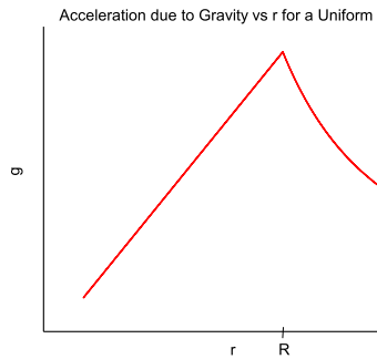
Figure 54.1: Acceleration due to gravity for a uniform sphere.
