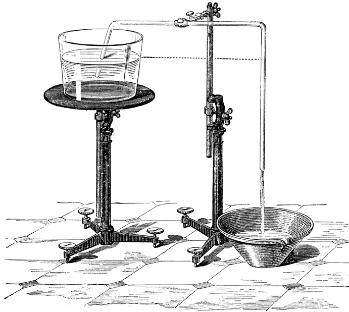
Figure 52.3: A siphon. (From Ref. [16])
