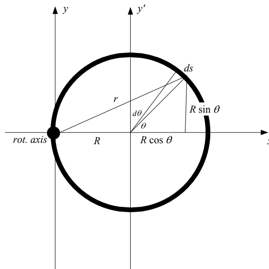
Figure 37.3: Calculation of the moment of inertia of a hoop when rotated about an axis passing through the hoop.
