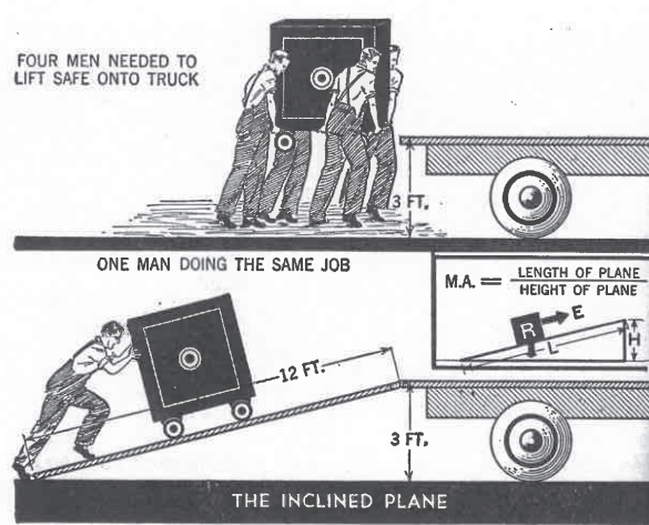
Figure 25.1: The inclined plane. In this example, L = 12 ft, H = 3 ft, so the mechanical advantage is M.A. = L/H = 4 . Rolling the safe up the incline requires only 1/4 the force of lifting it directly. (Ref. [19])
