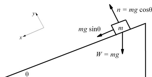
Figure 17.1: An object sliding on an inclined plane.
