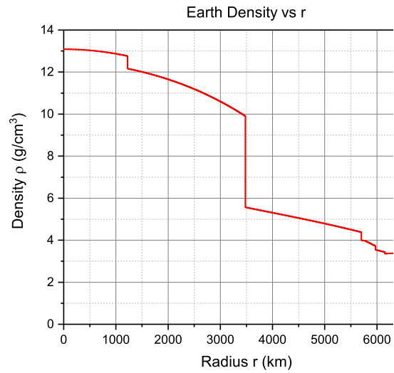
Figure 54.2: Earth density model (Dziewonski and Anderson, 1981.)
