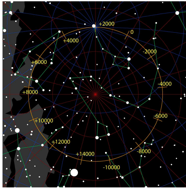
Figure 55.1: Star chart showing the direction of the Earth's north pole for different years. The movement is due to precession of the Earth's axis, and has a period of about 26,000 years. (Credit: Tau'olunga, Wikipedia.)
