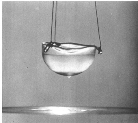
Figure 52.6: A Rollin film of superfluid helium II. The film creeps up the sides of the container and back down the outside, collecting in small drops at the bottom. ( Credit: Liquid Helium II: The Superfluid, University of Michigan. )
