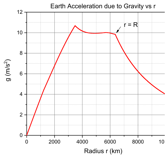
Figure 54.3: Modeled acceleration due to gravity for Earth.
