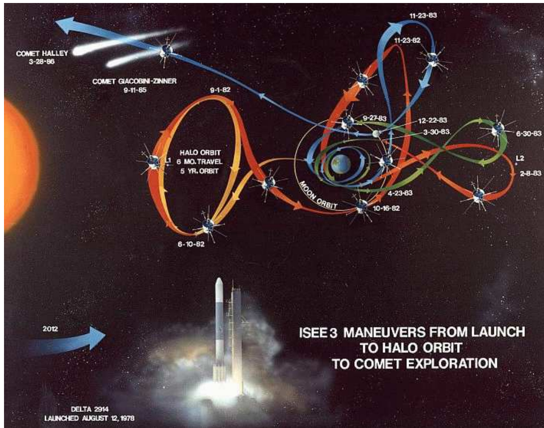
Figure 58.5: In 1982, the International Sun/Earth Explorer 3 (ISEE-3) spacecraft was re-purposed to become the International Cometary Explorer (ICE), so that it could explore comets Giacobini-Zinner and Halley. ISEE-3 orbited the L_1 Sun-Earth Lagrange point. Getting the spacecraft to intercept the two comets involved one of the most complex trajectories ever designed (shown here). (Credit: NASA.)
