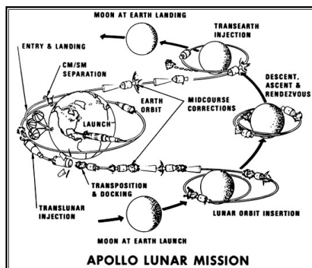
Figure 58.4: Orbits of Apollo spacecraft 8 and 10–17. The spacecraft enters lunar orbit in front of the Moon, to help slow its velocity. (Credit: NASA.)
