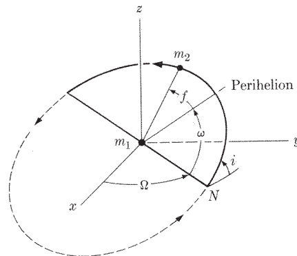
Figure 57.1: Orbital elements for a body of mass m_2 orbiting a body of mass m_1 . The xy -plane is the reference plane, and x is the direction of the vernal equinox. Shown are the orbital elements i , \Omega , and \omega , along with the true anomaly f . Point N is the ascending node of the orbit. (From McCuskey, 1963 [14].)
