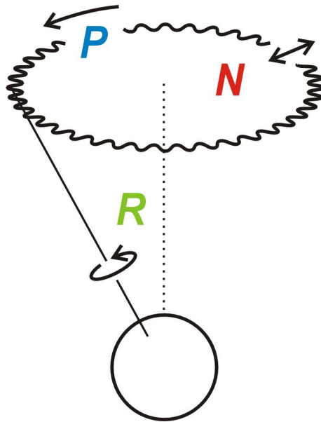
Figure 55.2: Precession ( P ) and nutation ( N ) of the Earth's rotation axis R . The nutation is a small “nodding” motion superimposed on the larger precessional motion. This figure shows the general shape of the nutation, with a period of about 18.6 years; the actual motion, when seen in detail, is more complex. (Credit: ©GNU-FDL, Wikimedia Commons.)
