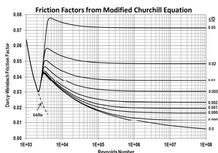
Figure 52.4: Friction factor as a function of Reynolds number, for both laminar and turbulent flow. (Ref. [13])
