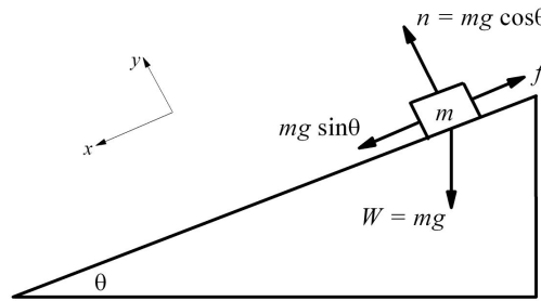
Figure 20.1: An object sliding on an inclined plane, with friction included.
