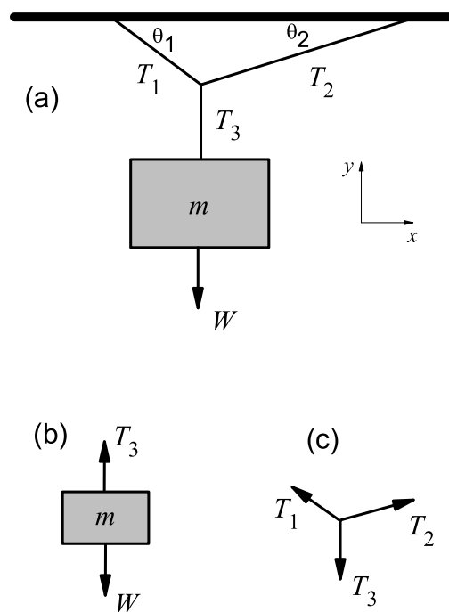
Figure 19.1: A block suspended from the ceiling by ropes. (a) Diagram of the situation. The block of mass m is suspended by a rope; the upper end of the rope is attached to two other ropes that are attached to the ceiling. (b) Free-body diagram for the block. (c) Free-body diagram for the knot.
