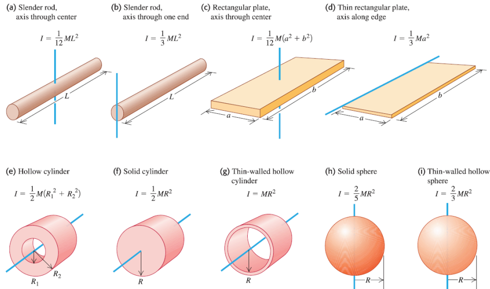
Figure 37.4: Table of moments of inertia of uniform bodies. (Credit: University of Pennsylvania.)
