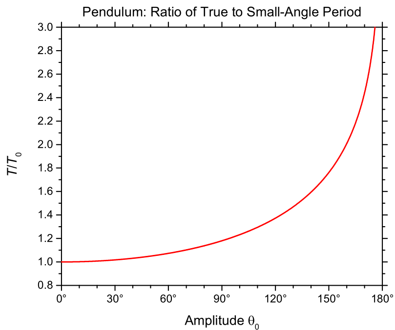
Figure 20.1: Ratio of a pendulum's true period T to its small-angle period T_0 = 2\pi \sqrt{L/g} , as a function of amplitude \theta_0 . For small amplitudes, this ratio is near 1; for larger amplitudes, the true period is longer than predicted by the small-angle approximation.
