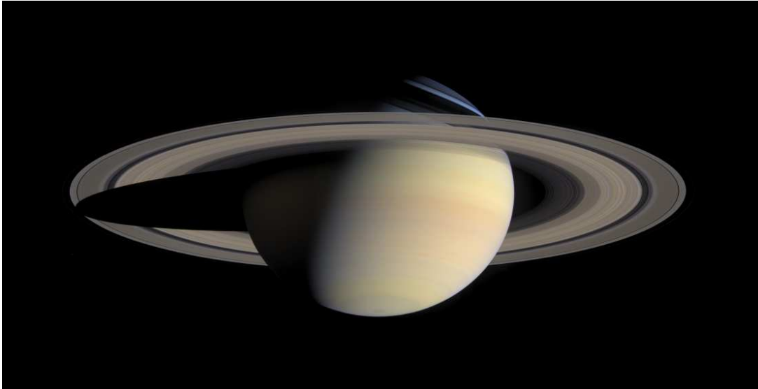
Figure 57.3: Saturn and its rings, as seen by the Cassini spacecraft. (Credit: NASA.)
