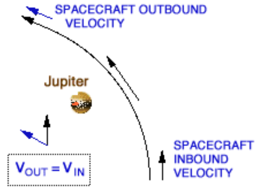
Figure 58.2: Spacecraft flying past a stationary Jupiter. Credit: NASA Jet Propulsion Laboratory.
