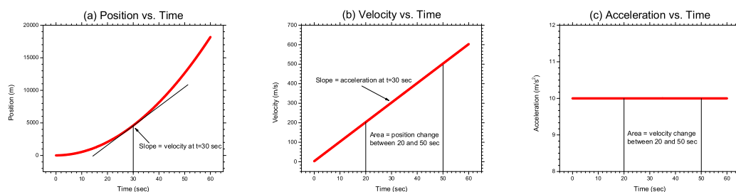
Figure 8.1: Plots of position, velocity, and acceleration vs. time for a particle moving according to x(t) = 5t^2 + 3t + 7 \text{ m} . From the calculus, we find (b) v(t) = dx/dt = 10t + 3 \text{ m/s} , and (c) a(t) = dv/dt = 10 \text{ m/s}^2 . The same results are found geometrically, as described in the text.
