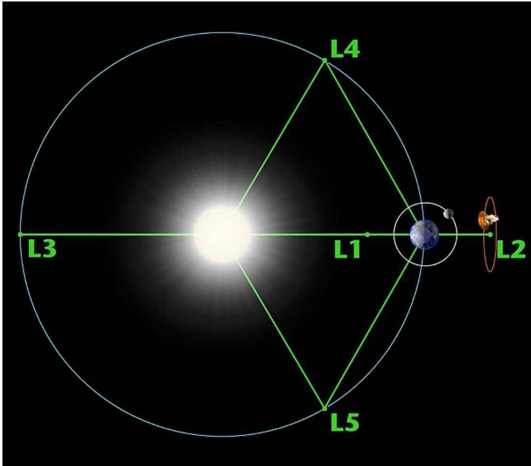
Figure 57.2: The Sun-Earth Lagrange points. The Wilkinson Microwave Anisotropy Probe (WMAP) spacecraft is shown orbiting the L_2 Lagrange point in a halo orbit. (Credit: NASA.)
