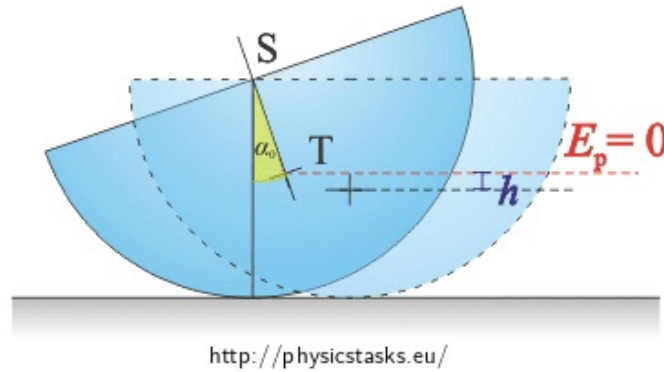
Figure 43.2: Rocking cylinder rocked by angle \alpha_0 .
