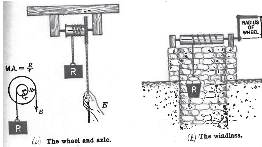
Figure 25.2: (a) The wheel and axle. (b) The windlass, another type of wheel and axle. Here R is the resistance (resistive force) and E is the effort (effort force). (Ref. [19])
