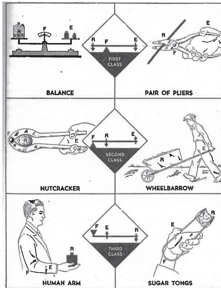
Figure 25.4: The three classes of levers. (Ref. [19])
