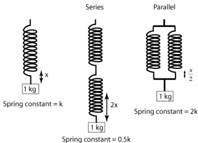
Figure 42.3: Springs in series and parallel (Credit: http://spmphysics.onlinetuition.com.my ).
