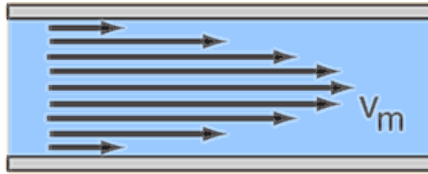
Figure 52.1: Laminar fluid flow through a pipe. The maximum flow velocity v_m is at the centerline and is equal to twice the average flow velocity. (Figure from Georgia State University, http://hyperphysics.phy-astr.gsu.edu/hbase/pfric2.html )
